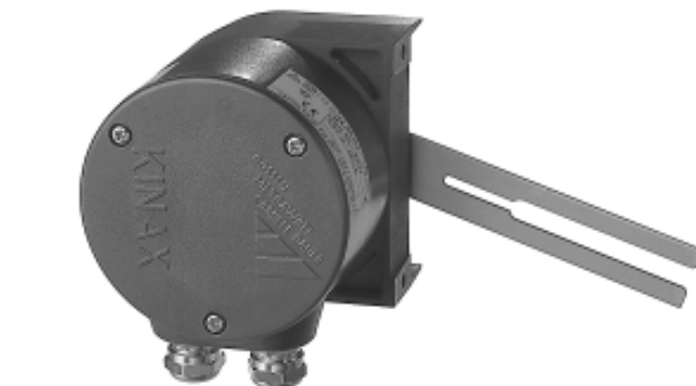
Fig. 1. Position feedback transmitter KINAX SR 709 showing the operating lever in the lower zero position, corresponding output current 0/4 mA.
