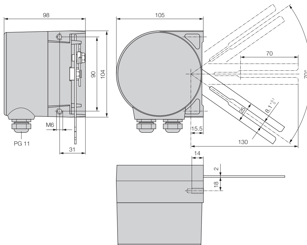
Fig. 7. Position of the KINAX SR 709 operating lever in the lower zero position, corresponding output current 0/4 mA.
