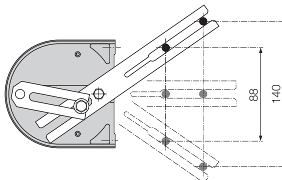
Fig. 4. Operating lever set for maximum operating angle.
