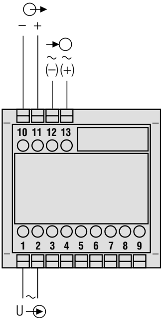
Fig. 5. Power supply connected to the low tension terminal side 12 and 13.
