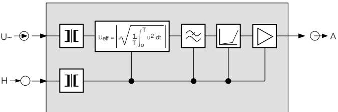
Fig. 2. Block diagram.
